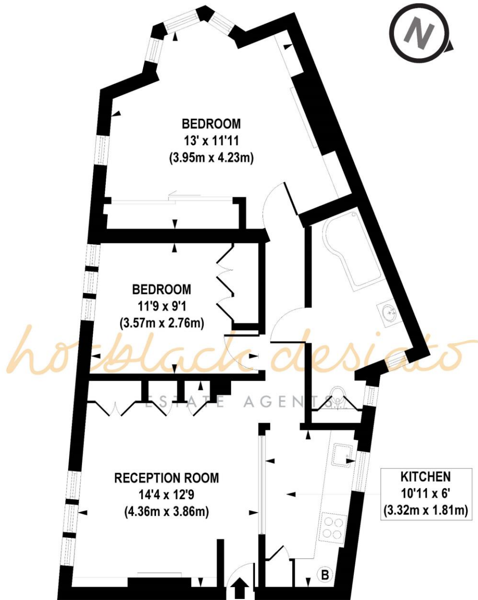
FIRST FLOOR
