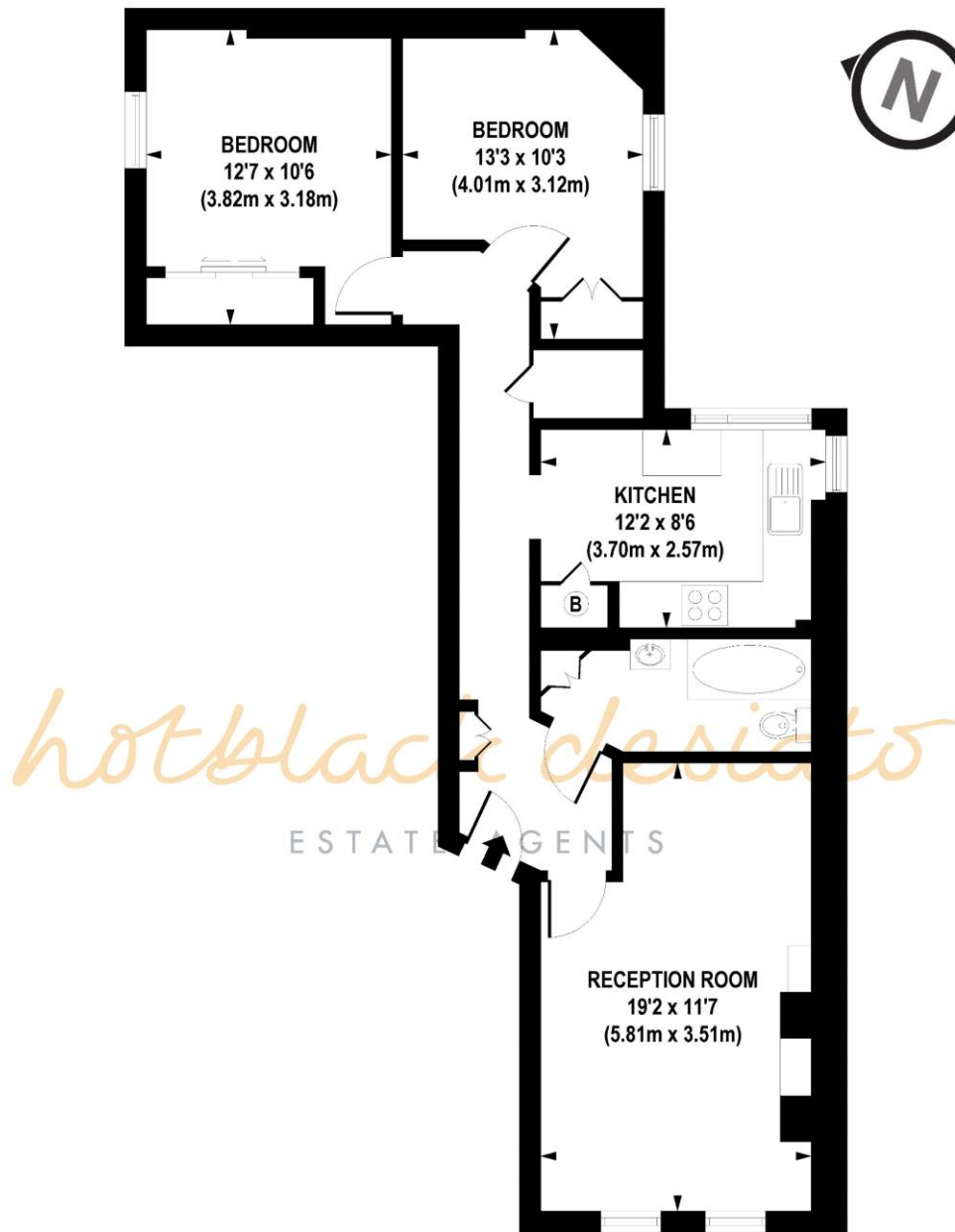
THIRD FLOOR
